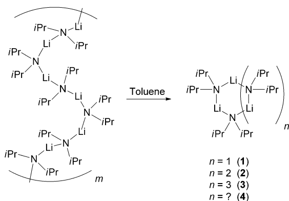
Scheme 1. LDA in the solid state and in toluene solution.
