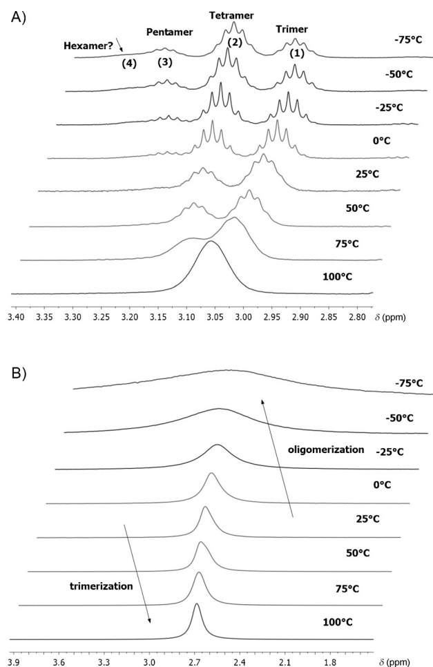
Figure 1. ^1\text{H} NMR spectra (A; \alpha\text{-CH} signals) and ^7\text{Li} NMR spectra (B) of LDA in [\text{D}_8]\text{toluene} at various temperatures.
